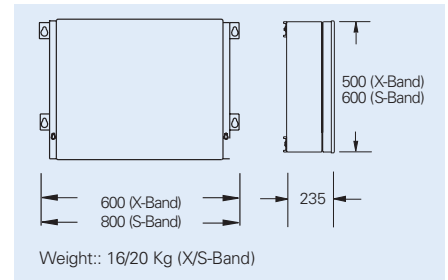
Bulkhead transceiver , type NG3040 (X-Band) and NG3041 (S-Band)
